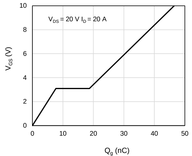
Figure 10: Gate-Charge Characteristics
